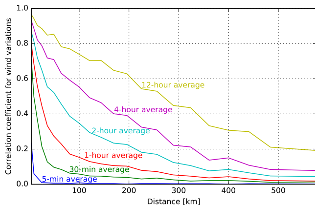
Figure 2: Correlation of variations in wind for different time scales in Germany. (Reproduced with permission and data from [110, 111])
