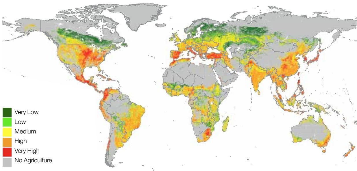
Global Insecticide Risk Potential map. The map shows the spatial distribution of potential insecticide runoff to stream ecosystems. According to this estimation, the surface waters in 43% of the total global land area are potentially subject to insecticide load as a consequence of current agricultural practices. The class boundaries (-3; -2; -1; 0) are the same as those used to previous studies (kattwinkel et al, 2011). Grey areas indicate the absence of any relevant agricultural activity. Reprinted from Environmental Pollution, 198, Ippolito, A., Kattwinkel, M., Rasmussen, J. J., Schäfer, R. B., Fornaroli, R. & Liess, M., Modeling global distribution of agricultural insecticides in surface waters, pages 54-60, Copyright (2015), with permission from Elsevier.
